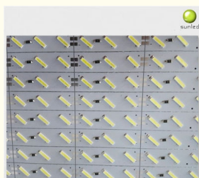
8520led rigid strip72leds/pcs
